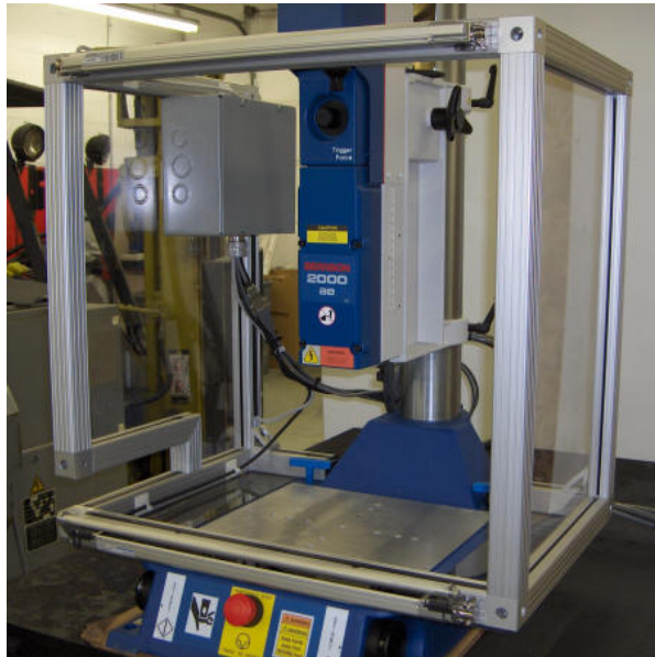
LCSS - PAT Light Curtain Safety-Start System
